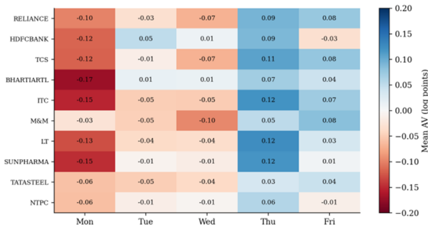
Figure 1: Mean Abnormal Volume by Weekday and Company
