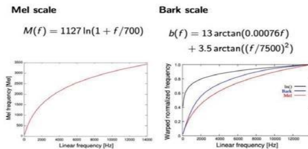
Figure 7: Frequency scale
